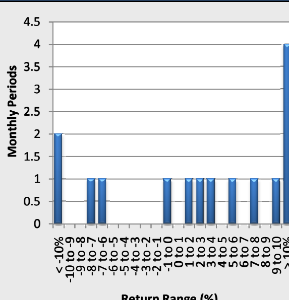
Distribution of Returns
